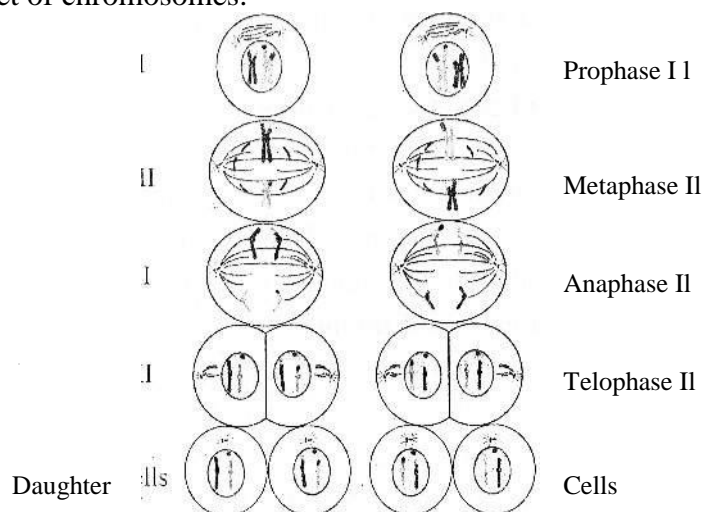
Figure 5.9: Stages in Meiosis-II
